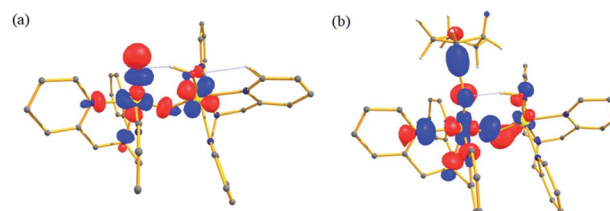
Fig. 9 Computed orbital diagram corresponding to the (a) LUMO of the {}^21_{\text{ns-hs}} and (b) HOMO of the 1\text{-}^2\text{TS}_{\text{Hns-hs}} .
