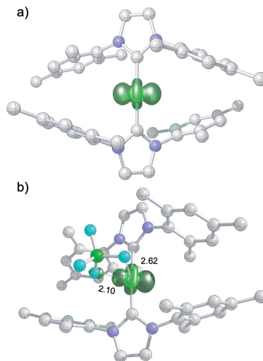
Fig. 5 (a) Spin density plot for [\text{Ni}(\text{Mes}_2\text{Im})_2]^+ ; (b) molecular structure of \mathbf{8}_{\text{DFT}}^1 showing Ni– \text{F}^{\text{BF}_4^-} contacts (isovalue \pm 0.0075 a_0^{-3} ; lengths of Ni–F contacts in \text{\AA} ; hydrogen atoms not shown).
