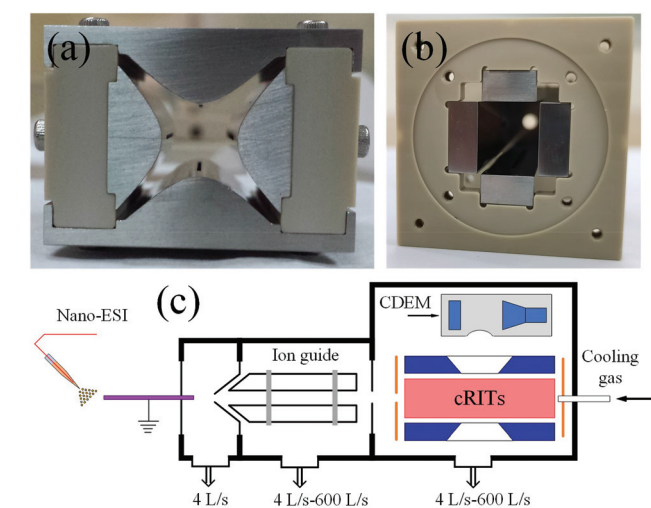
Fig. 1 (a) Photograph of the hyperbolic linear ion trap, (b) photograph of the ceramic-based rectilinear ion trap, and (c) the schematic of the digital ion trap mass spectrometer.
