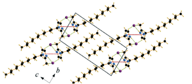
Fig. 5 Packing diagram of \text{C}_{12}\text{C}_1\text{C}_0 . Projection on the bc plane. \text{C}_g - \text{C}_g contacts are shown by red and \text{Br}\cdots\text{H} bonds by green dashed lines.
