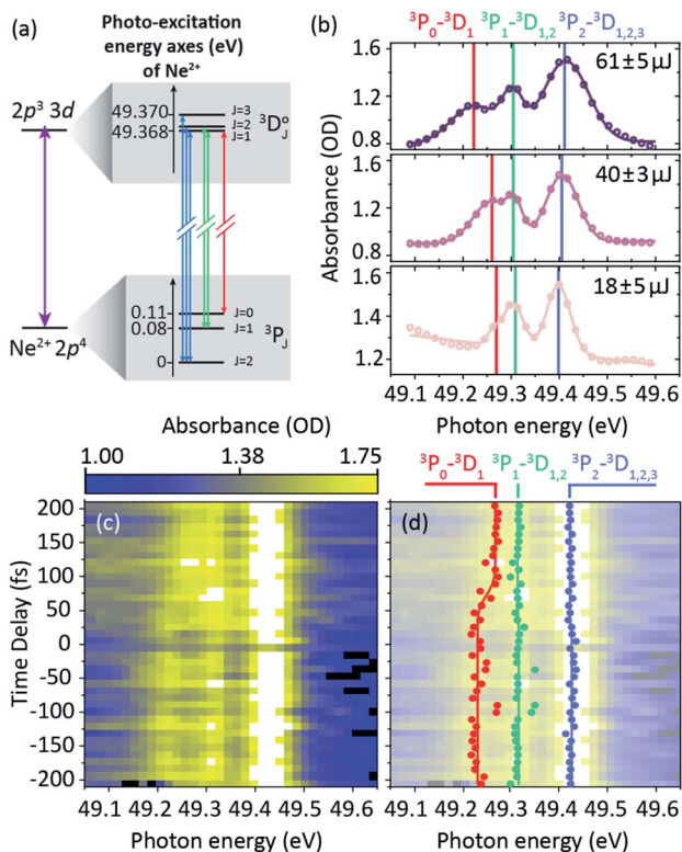
Fig. 7 (a) Level scheme of the resonant coupling mechanism of the Ne 2+ ion. Observed absorption lines correspond to the ground-state splitting, while the 1 meV-scale excited-state splitting is unresolved. The observed sets of multiplet transitions are indicated in blue, green, and red. (b) Static absorption spectroscopy of the pump pulse evaluated at large negative delays (probe first) for the mean pulse energies 18 \pm 5 \mu\text{J} (pulse-energy range <25 \mu\text{J} ), 40 \pm 3 \mu\text{J} (pulse-energy range 35\text{--}45 \mu\text{J} ), and 61 \pm 5 \mu\text{J} (pulse-energy range >55 \mu\text{J} ). Also see ref. 3 for further details on the experiment. (c) Time-resolved absorption data of the pump pulse at 69 \pm 3 \mu\text{J} mean pulse energy (pulse-energy range indicated in dark violet in Fig. 5b). (d) Fitted spectral positions of the observed lines (data points) and error-function fit to the fit results over time delay (corresponding solid lines) to find temporal duration and position of the transient spectral shift.
