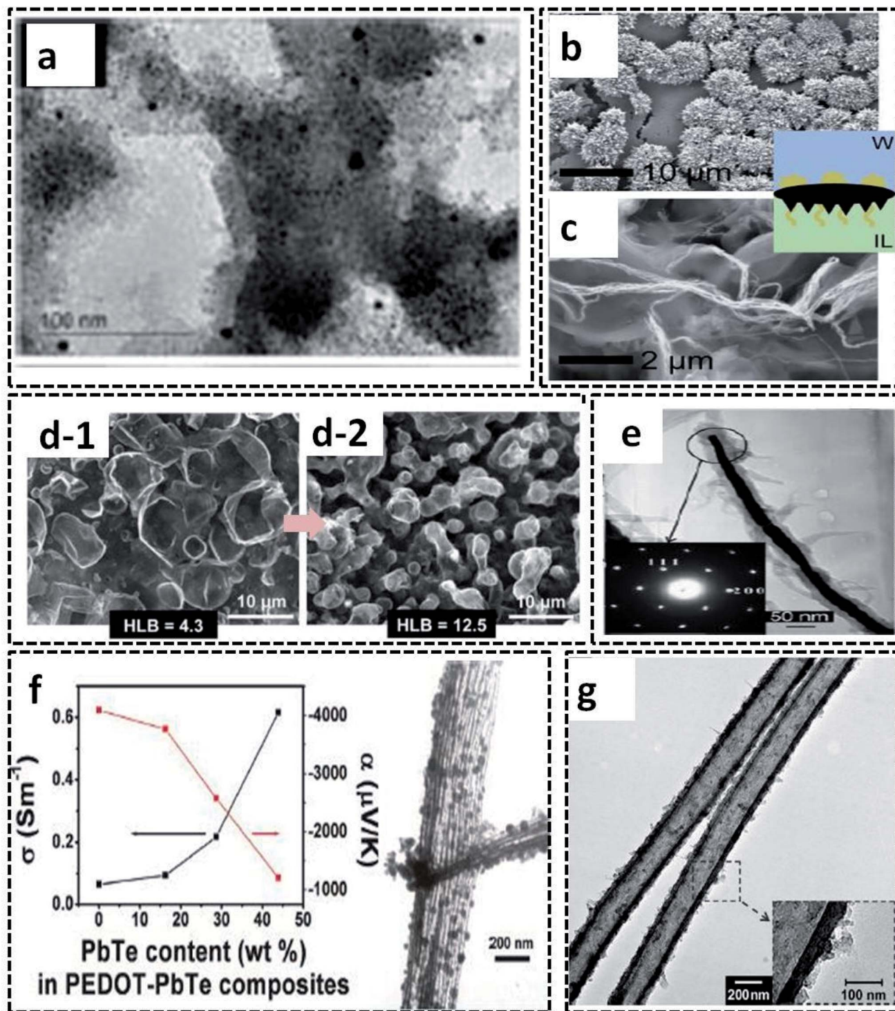
Fig. 10 (a) TEM images of the PTh/Au film. Reprinted from ref. 102, Copyright (2018), with permission from Elsevier. SEM images of (b) microroughin and (c) dendrite-like fiber shapes of the PTh/Au composite prepared by ionic liquid/water interfacial polymerization. Reprinted with permission from ref. 21. Copyright (2018) American Chemical Society. (d) SEM images of PPY synthesized by water/chloroform interface-assisted polymerization in the presence of a surfactant mixture (Span 80 and OP 10). The transformation of the morphology from a ruptured vesicle type to coral type is shown in the figure with an arrow. Reprinted from ref. 104, Copyright (2018), with permission from Elsevier. (e) TEM image of PEDOT/Au nanocable with inset showing the SAED pattern of the highly crystalline Au. Reprinted with permission from ref. 2. Copyright (2007) American Chemical Society. (f) TEM image of the PEDOT-PbTe composite tubes showing thermoelectric property. Reprinted with permission from ref. 105. Copyright (2011) American Chemical Society. (g) The TEM image of the 1-D PEDOT nanotubes prepared by water in oil micro-emulsion interfacial polymerization method. Reproduced with permission under a Creative Commons CC-BY License from ref. 106. Copyright 2007 John Wiley and Sons.
