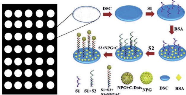
Fig. 28 The CD-based CL sensor for the detection of DNA. Figure reproduced from ref. 283 with permission from Royal Society of Chemistry, copyright 2013.
