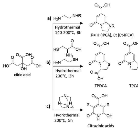
Scheme 1 Molecular fluorophores identified in the synthesis of CA-derived CDs using different amino-containing precursors: (a) ethylene diamine, 204 (b) cysteine and cysteamine, 205 and (c) hexamethylenetetramine. 207
