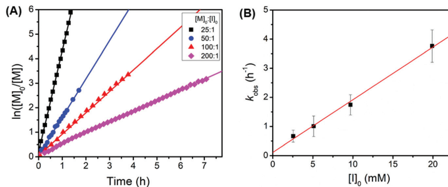
Fig. 4 (A) Plots of \ln([M]_0/[M]_t) versus time butylamine-initiated ROPs of {}^t\text{BuO}_2\text{Pr-NCA} in toluene at room temperature with a constant initial monomer concentration and varying initiator concentration (i.e., [M]_0 = 0.5\text{ M} , [M]_0:[I]_0 = 25:1, 50:1, 100:1 , and 200:1 ), and (B) the pseudo-first order observed polymerization rate constant ( k_{\text{obs}} , ■) versus the initial initiator concentration ( [I]_0 ) and the linear fit (—) of the data, the slope of which yields the propagation rate constant k_p = 181 \pm 8\text{ M}^{-1}\text{ h}^{-1} .
