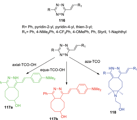
Scheme 25 Reaction of styryltetrazines 116 with two TCO-OH isomers and aza-TCO.
