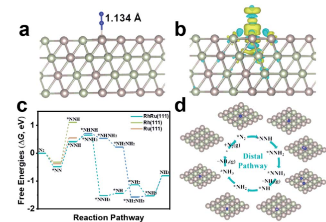
Fig. 4 (a) The optimized structure of N 2 adsorbed vertically on the Ru top site of the RhRu(111) surface in side view. (b) Difference charge density of N 2 adsorption on the RhRu(111) surface with a Rh : Ru atom ratio of 1 : 1. The yellow and cyan regions represent electron accumulation and depletion, respectively, and the isosurface value is 0.0012 e bohr -3 . (c) Calculated free energy diagrams for N 2 electro-reduction on the RhRu(111) surface with a Rh : Ru atom ratio of 1 : 1 in a 4 × 4 supercell. (d) The optimized intermediates by the distal pathway in top view. The adsorption site is denoted by an asterisk (*) and the H, N, Rh and Ru atoms are shown in pink, blue, yellow and brown colors, respectively.
