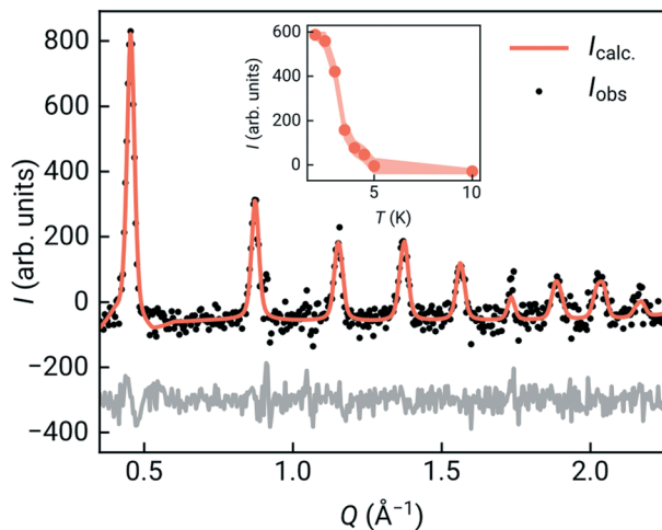
Fig. 3 Detail of the magnetic Rietveld refinement on the P_{21/n} Shubnikov space group, showing all observed magnetic Bragg peaks. The magnetic contribution has been isolated by subtracting the paramagnetic contribution (10 K). Observed (black points) and calculated (orange solid line) powder diffraction pattern (magnetic R_{\text{Bragg}} = 7.77 ). The observed-calculated difference pattern is depicted as a grey line at the bottom of the figure. Inset depicts the temperature dependence of the intensity of the first observed magnetic Bragg line obtained through Gaussian fitting of a single line.
