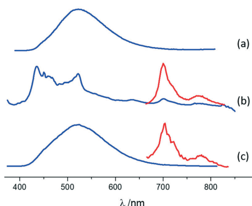
Fig. 6 Normalized luminescence spectra in the solid state of (a) pure MA, (b) MA \cdot I2F4 , and (c) (MA)_4 \cdot I2F4 (arbitrary units on the y-axis). \lambda_{\text{exc}} = 380 \text{ nm} . The phosphorescence spectra in the 650–850 nm region, isolated with a gated detection, are magnified in the inset for MA \cdot I2F4 and (MA)_4 \cdot I2F4 . In both co-crystals the phosphorescence emission is clearly evidenced compared to the parent PAH 9-methylanthracene, where no phosphorescence was detected at all. Moreover, for MA \cdot I2F4 the spectrum is not dominated by excimer emission.
