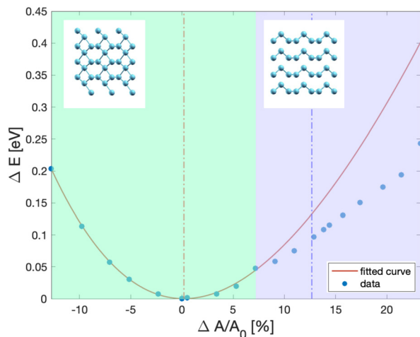
Fig. 4 Energy (dots) per unit cell (three atoms per cell) versus surface area of the \text{Te}(10\bar{1}0) trilayer slab from DFT calculations. The surface area is expressed in variation in % with respect to the area at the minimal energy ( 4.142 \times 5.449 \text{ \AA}^2 , see text). The red line is a fitting of the data with a 2D version of the Birch–Murnaghan equation of state. In the green region the system is in the \beta geometry of ref. 8, while in the violet region the bulk-like helical chains are recovered. The insets show the crystal structure in the two regimes. The blue dashed line corresponds to the DFT equilibrium unit cell area of a \text{Te}(10\bar{1}0) double-trilayer from ref. 28.
