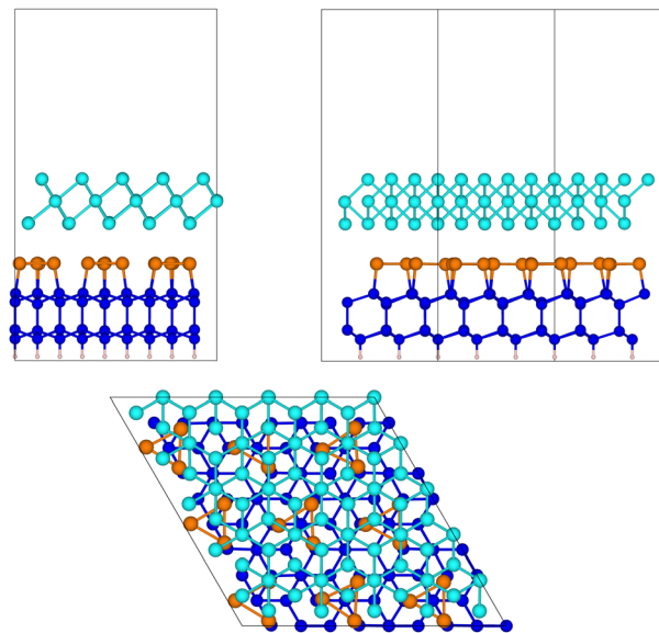
Fig. 5 The relaxed configuration of tellurene in a trilayer 1T- \text{MoS}_2 -like geometry adsorbed on the \text{Si}(111)-(\sqrt{3} \times \sqrt{3})R30^\circ -Sb surface in a slab geometry. Side and top views are shown.
