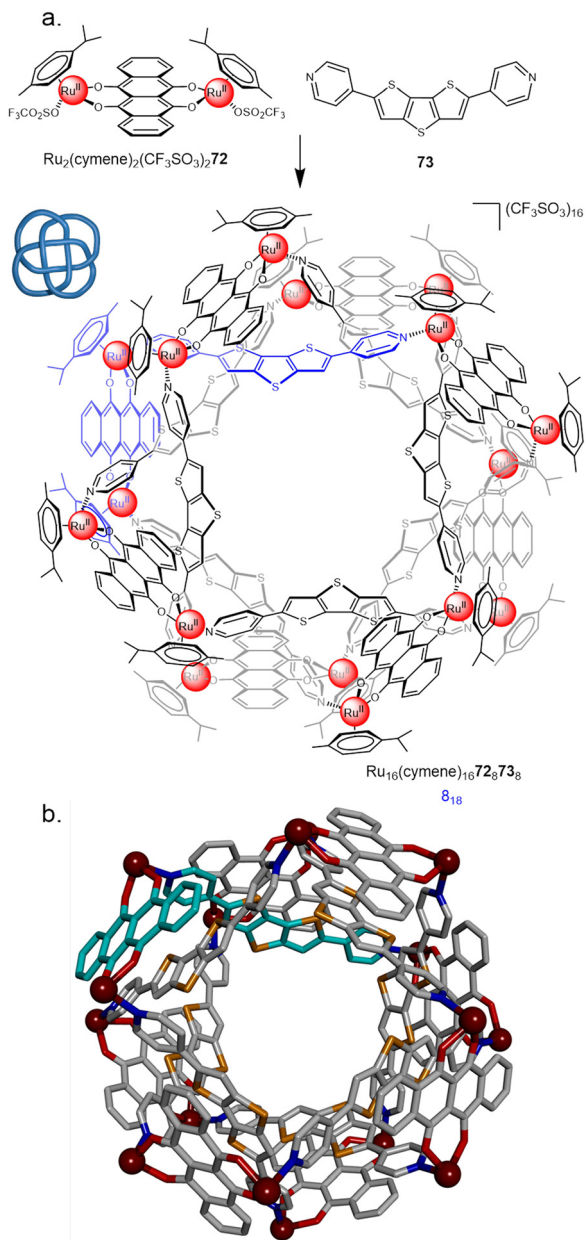
Fig. 25 (a) Synthesis of \text{8}_{18} metalla-knot \text{Ru}_{16}(\text{p-cymene})_{16}\text{72}_8\text{73}_8 . (b) X-ray crystal structure of the \text{8}_{18} metalla-knot with p -cymene ligands omitted for clarity. 100
