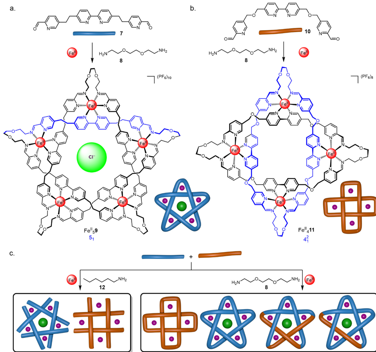
Fig. 5 Self-assembly of (a) molecular pentafoil knot 43 Fe II 5 9 and (b) Solomon link 45 Fe II 4 11 using dynamic imine exchange. (c) Self-sorting of circular helicates, knots and links. 46
