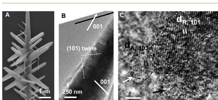
Fig. 6 Ex situ TEM data showing (A) a branched rutile nanowire, (B) the crystallographic relationship between the branches and trunk, and (C) attachment of the (103) faces of anatase nanoparticles onto the (101) faces of rutile nanowires, followed by transformation to rutile. 48 Reprinted with permission from ref. 48. Copyright 2013 American Chemical Society.
