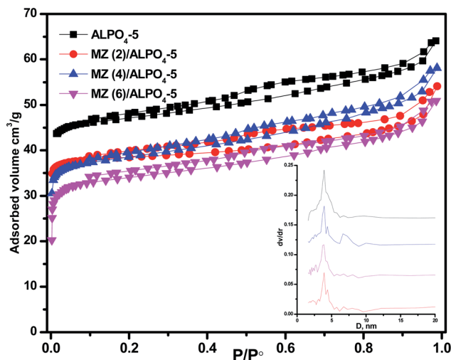
Fig. 2 \text{N}_2 adsorption/desorption isotherms of MZn ( x )/ \text{AlPO}_4 -5 nanocomposites, x = 0, 2, 4 , and 6. The inset is the pore size distribution of the prepared nanocomposites.
