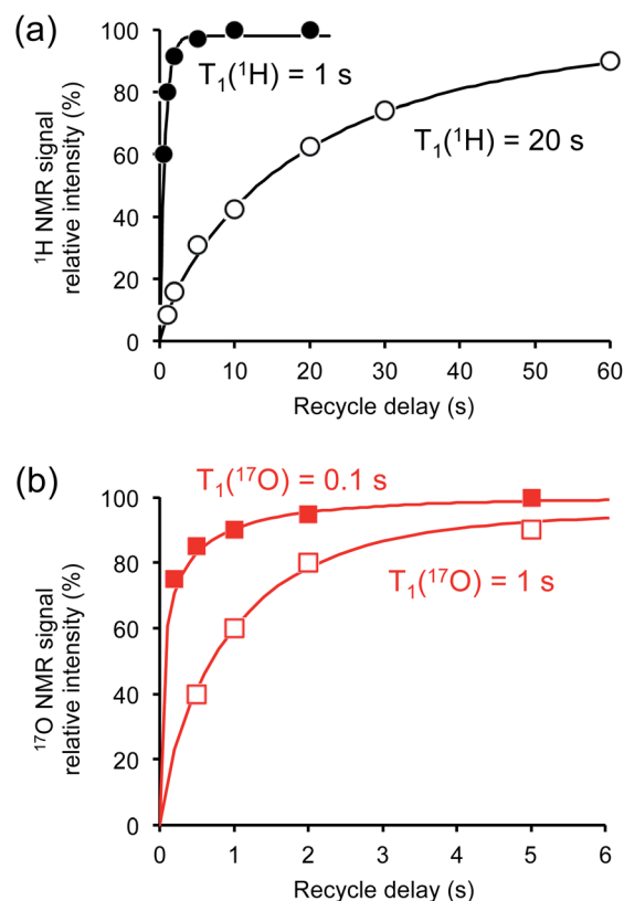
Fig. 6 Effects of paramagnetic Cu(II)–EDTA doping on (a) ^1\text{H} and (b) ^{17}\text{O} spin–lattice relaxation times. All measurements were carried out at 14.1 T for the [2\text{-}^{17}\text{O}]\text{-}\alpha\text{-D-glucose}/\text{NaCl}/\text{H}_2\text{O} cocrystal with (closed symbols) and without (open symbols) added Cu–EDTA.
