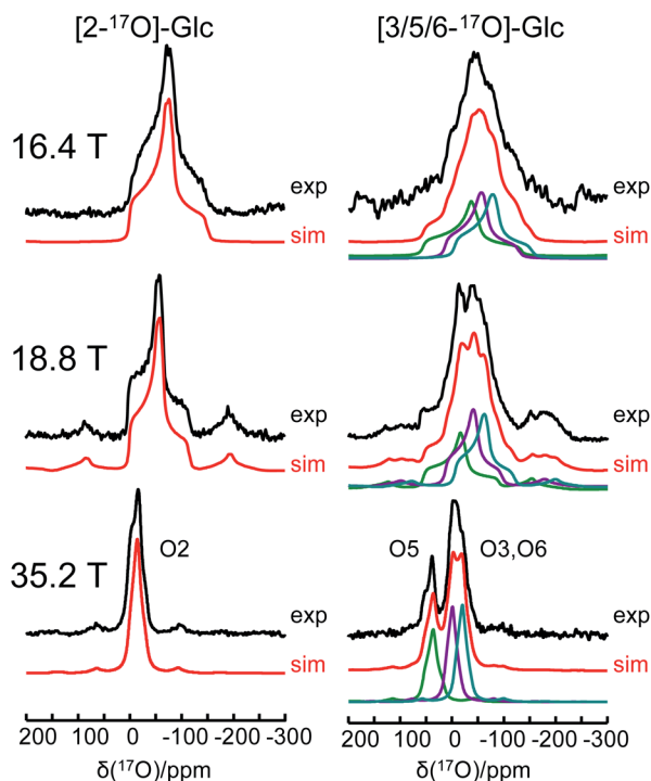
Fig. 5 Experimental (black traces) and simulated (red traces) ^{17}\text{O} MAS NMR spectra of [2\text{-}^{17}\text{O}]\text{-}\alpha\text{-D-glucose} and [3/5/6\text{-}^{17}\text{O}]\text{-}\alpha\text{-D-glucose} at three magnetic fields.
