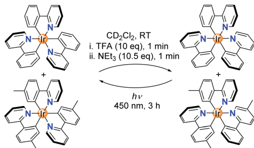
Scheme 3 A fac → mer → fac isomerization sequence with a mixture of Ir(pppy) 3 and Ir(tppy) 3 does not lead to ligand scrambling.
