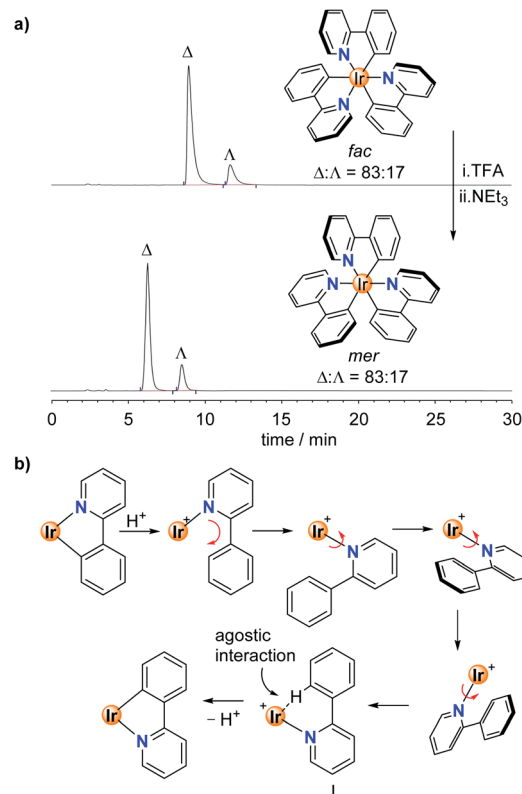
Fig. 3 (a) HPLC profile of a sample containing enantio-enriched fac -Ir(pppy) 3 before (top) and after (bottom) acid-base-induced fac → mer isomerization. (b) Plausible mechanism for the isomerization involving an in-plane movement of the protonated Hppy ligand and a 180° rotation around the Ir–N bond. A sequential movement–rotation is shown for illustrative purposes.
