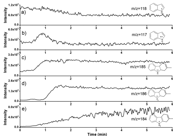
Fig. 4 Dynamic studies of different ions in confined spaces. EICs of [1 + \text{H}]^+ at m/z 118 (a), 1^{+\cdot} at m/z 117 (b), 3^{+\cdot} at m/z 185 (c), [3 + \text{H}]^+ at m/z 186 (d), and [4 + \text{H}]^+ at m/z 184 (e).
