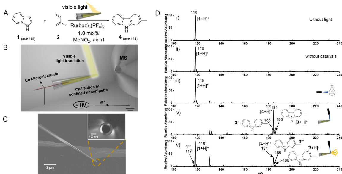
Fig. 1 (A) Scheme of the indole cation-radical cyclization catalyzed by \text{Ru}(\text{bpz})_3(\text{PF}_6)_2 (1% eq.) under mild conditions. (B) Schematic diagram of nanopipette-based photocatalytic reactor and in situ monitoring system associated with in situ nanoESI-MS. (C) SEM images of nanopipette and the orifice (the inset). (D) Mass spectrometric analysis of Ru-catalyzed indole cation-radical cyclization under different conditions. Indole cation-radical cyclization in nanopipette without light irradiation (i) or without catalyst (ii), in normal flask (iii), nanopipette (iv) and microdroplets (v). All spectra were collected after reacting for 20 s.
