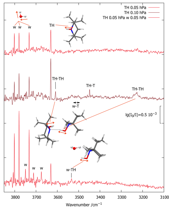
Fig. 2 FTIR spectra of TH with varying traces of T (<10%, based on CH signals, see ESI † ) and w co-expanded in 750 hPa helium (darker red illustrates higher TH concentration). The OH stretching absorptions of TH, TH–TH and w–TH are marked, as are a few rotational transitions of the water monomer antisymmetric OH stretch (w) which become more visible with increasing water concentration. 22
