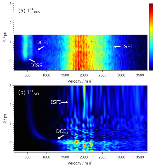
Fig. 15 2-D false-colour maps comparing the I^{3+} ion velocities following 267 nm photolysis of CH_3I and probing with (a) an 11.5 nm XUV pulse and (b) 805 nm SFI with I \sim 1300 \text{ TW cm}^{-2} (after subtraction of the NIR-only contribution), illustrating the very different relative weights of the DISS and DCE_3 signal contributions in the two cases. The relative intensities in both panels are depicted using the linear false-colour scale shown to the right of panel (a).
