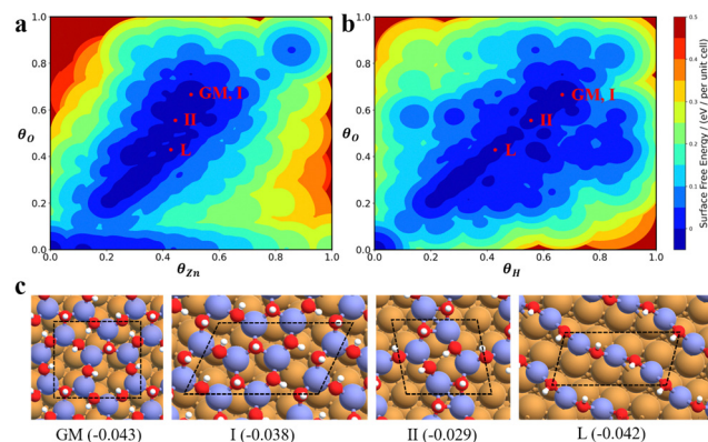
Fig. 8 The PES contour map for Zn x O y H z /Cu(111) from ASOP simulation, using (a) coverage of O and Zn as axes, or (b) coverage of O and H as the axes. (c) The identified stable Zn x O y H z /Cu(111) structures. From left to right, GM: Zn 6 O 8 H 8 /Cu(111) – (2√3 × 3), I: Zn 6 O 8 H 8 /Cu(111) – (√19 × √7), II: Zn 4 O 5 H 5 /Cu(111) – (3 × √7), L: Zn 3 O 3 H 3 /Cu(111) – (√13 × √3). The color scheme for atoms is as follows: H: white; O: red; Cu: yellow; and Zn: blue.
