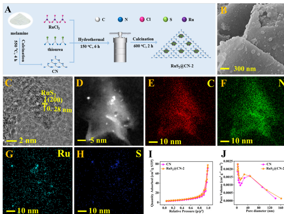
Fig. 1 Preparation scheme of RuS 2 @CN- x (A). SEM image (B) and TEM images (C and D) of RuS 2 @CN-2. Elemental mapping images of RuS 2 @CN-2: C (E), N (F), Ru (G), S (H). N 2 adsorption–desorption isotherms of CN and RuS 2 @CN-2 (I). Pore width distribution of CN and RuS 2 @CN-2 (J).
