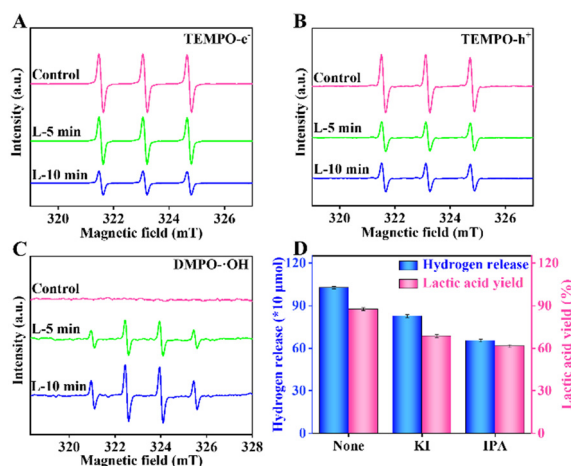
Fig. 6 TEMPO ESR spin-labelling for e^- (A) and h^+ (B) of \text{RuS}_2@\text{CN}-2 . DMPO ESR spin-labelling for \cdot\text{OH} of \text{RuS}_2@\text{CN}-2 (C). The effects of different oxidation active species on the photocatalytic performances (D).
