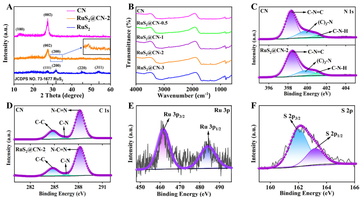
Fig. 2 XRD patterns of CN, RuS 2 @CN-2, and RuS 2 (A). FT-IR spectra of as-prepared samples (B). XPS high-resolution spectra of CN and RuS 2 @CN-2: N 1s (C), C 1s (D), Ru 3p (E) and S 2p (F).
