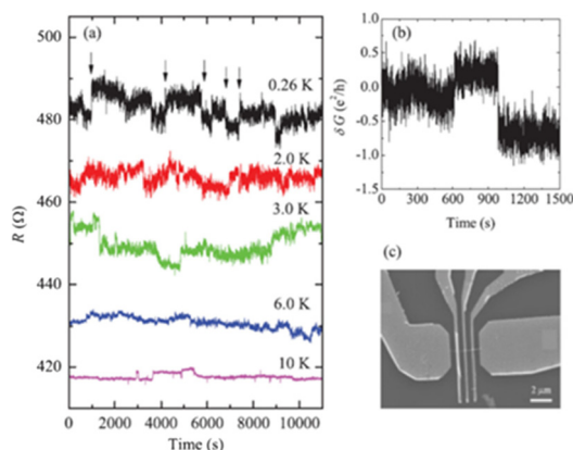
Fig. 16 (a) Resistance at five temperatures for a RuO_2 NW with length L = 1.5 \mu m and diameter d = 67 nm . Data at 6.0 K, 3.0 K, 2.0 K, and 0.26 K are offset by 10 \Omega , 20 \Omega , 30 \Omega , and 40 \Omega , respectively, for clarity. (b) Conductance variation \delta G = G - \langle G \rangle vs. time at 0.26 K. (c) Scanning electron microscope (SEM) image of lithographically defined NW. Reproduced from ref. 65 with permission. Copyright 2011 American Institute of Physics.
