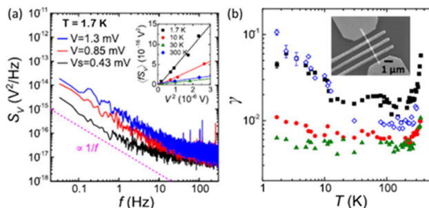
Fig. 17 (a) S_V vs. f and T for an IrO_2 NW with L = 0.9 \mu m and d = 147 nm ; \langle S_V \rangle vs. V^2 is shown in the inset. (b) \gamma = S_V N_c f / V^2 vs. T for IrO_2 NWs from 1.7 K to 350 K. The inset is a SEM image of a NW. Dimensions are L = 1.9 \mu m, d = 143 nm (solid black squares); L = 1.0 \mu m, d = 123 nm (solid red circles); L = 0.75 \mu m, d = 125 nm (solid green triangles); and L = 0.9 \mu m, d = 147 nm (open blue diamonds). Reproduced from ref. 75 with permission. Copyright 2023 American Institute of Physics.
