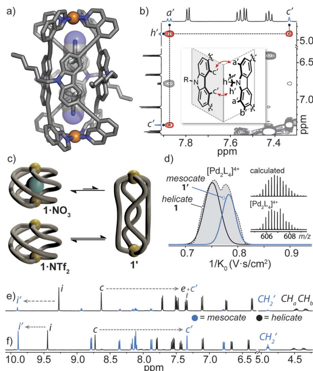
Fig. 5 (a) X-ray structure of mesocate 1' showing the MeCN solvent guests; (b) ^1\text{H} - ^1\text{H} NOESY spectrum of \mathbf{1}\cdot\text{NTf}_2 ( \text{R} = \text{C}_6\text{H}_{13} ), showing the important contacts in the inset; (c) a schematic of the anion-dependant equilibrium between the helicate 1 and mesocate 1' ; (d) Trapped Ion Mobility (TIMS) mobilogram alongside the measured and calculated isotope pattern of the 4+ species of \mathbf{1}\cdot\text{NTf}_2 ; (e) ^1\text{H} NMR spectra (500 MHz, \text{CD}_3\text{CN} ) of \mathbf{1}\cdot\text{NO}_3^- after 2 weeks at 25^\circ\text{C} (signal c' arising from 1' overlaps with signals of 1 ); (f) \mathbf{1}\cdot\text{NTf}_2 after two weeks at 25^\circ\text{C} .
