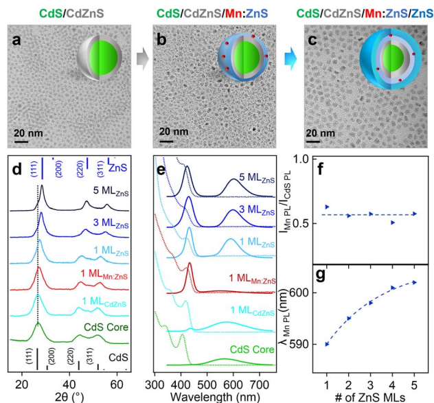
Fig. 3 (a–c) TEM images of CdS/CdZnS, CdS/CdZnS/Mn: ZnS, and CdS/CdZnS/Mn: ZnS/ZnS core/multi-shell QDs. (d) XRD patterns and (e) normalized absorption (dotted lines) and PL (solid lines) spectra of CdS core and CdS/CdZnS/Mn: ZnS/ZnS (1–5 MLs) core/multi-shell QDs. (f) The PL Intensity ratio of Mn(II) and CdS host lattice ( I_{Mn PL}/I_{CdS PL} ) and (g) the Mn(II) PL peak position as a function of ZnS shell thickness.
