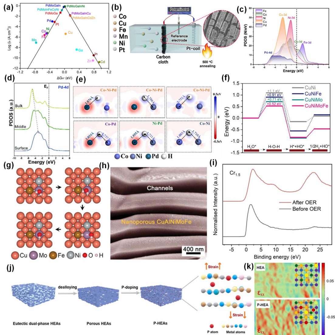
Fig. 6 (a) Volcano chart for the HER. Reproduced with permission. 91 Copyright 2022, American Chemical Society. (b) Loading Pt by electrodeposition. Reproduced with permission. 95 Copyright 2022, Wiley-VCH. (c) The PDOS. (d) The site-dependent PDOS of Pd. (e) DFT results of electron density difference between sites after H* adsorption. Reproduced with permission. 15 Copyright 2022, Elsevier Ltd. (f) Reaction energy diagram of water dissociation at different stages. (g) Surface configuration of the CuNiMoFe alloy. (h) SEM image of nanoporous CuAlNiMoFe. Reproduced with permission. 65 Copyright 2021, Wiley-VCH. (i) Normalized valence band spectra (VBS) of Cr 1.5 MnFeNi. Reproduced with permission. 45 Copyright 2023, Elsevier Ltd. (j) Composite diagram of P-HEA. (k) Strain maps of HEA and P-HEA. Reproduced with permission. 97 Copyright 2023, Elsevier Ltd.
