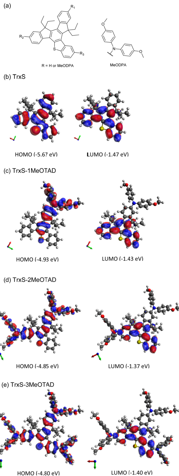
Fig. 2 (a) Molecular representation of the TrxS core and MeODPA substituent. Variations considered in the calculations were: R 1 = R 2 = R 3 = H (TrxS); R 1 = MeODPA and R 2 = R 3 = H (TrxS-1MeOTAD); R 1 = R 2 = MeODPA and R 3 = H (TrxS-2MeOTAD) and R 1 = R 2 = R 3 = MeODPA (TrxS-3MeOTAD). HOMO and LUMO of (b) TrxS, (c) TrxS-1MeOTAD, (d) TrxS-2MeOTAD and (e) TrxS-3MeOTAD in dichloromethane, calculated by B3LYP 6-311G(d).
