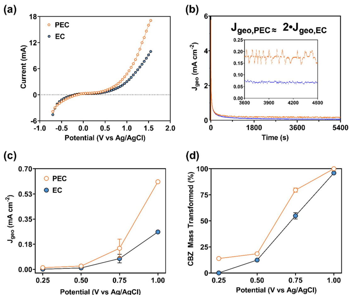
Fig. 6 For the optimal (0.45 g PAN/50 wt% \text{TiO}_2/1000 \text{ }^\circ\text{C} ) CNF/ \text{TiO}_2 composite: (a) average faradaic current resulting from staircase cyclic voltammetry (SCV; 50 mV, 30 s, -0.7 to 1.5 V) with and without light; (b) representative current density–time profiles for photoelectrochemical (PEC) and electrochemical (EC) transformation at +0.75 V vs. Ag/AgCl; (c) average faradaic current density during PEC and EC transformation (300–5400 s); and (d) CBZ mass transformed (%) during PEC and EC transformation (0–5400 s). Parameters: C_0 = 10 \mu\text{M} CBZ, 0.5 M phosphate buffer at pH 7.4.
