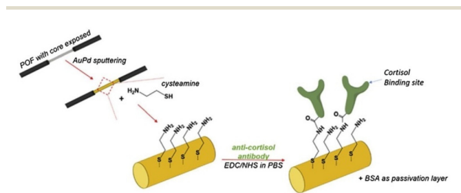
Fig. 11 Preparation of the Optical fiber. Reproduced from ref. 88 with permission from Elsevier, copyright 2021.
