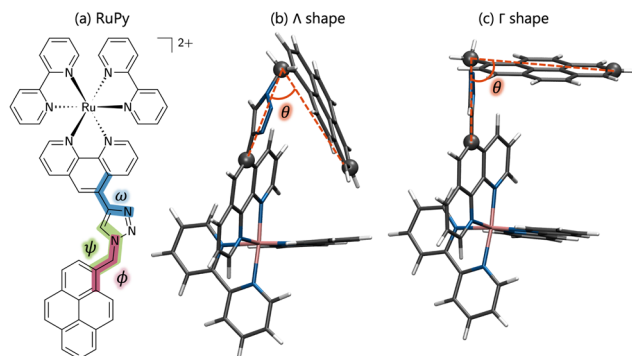
Fig. 1 (a) Structure of the ruthenium(II) complex (RuPy) depicting the \phi , \omega and \psi torsional angles in red, blue and green, respectively. (b) RuPy in the \Lambda -shaped geometry, and (c) \Gamma -shaped geometry. Color code for atoms and angle \theta : grey for C, blue for N, pink for Ru, white for H, and red for O.
