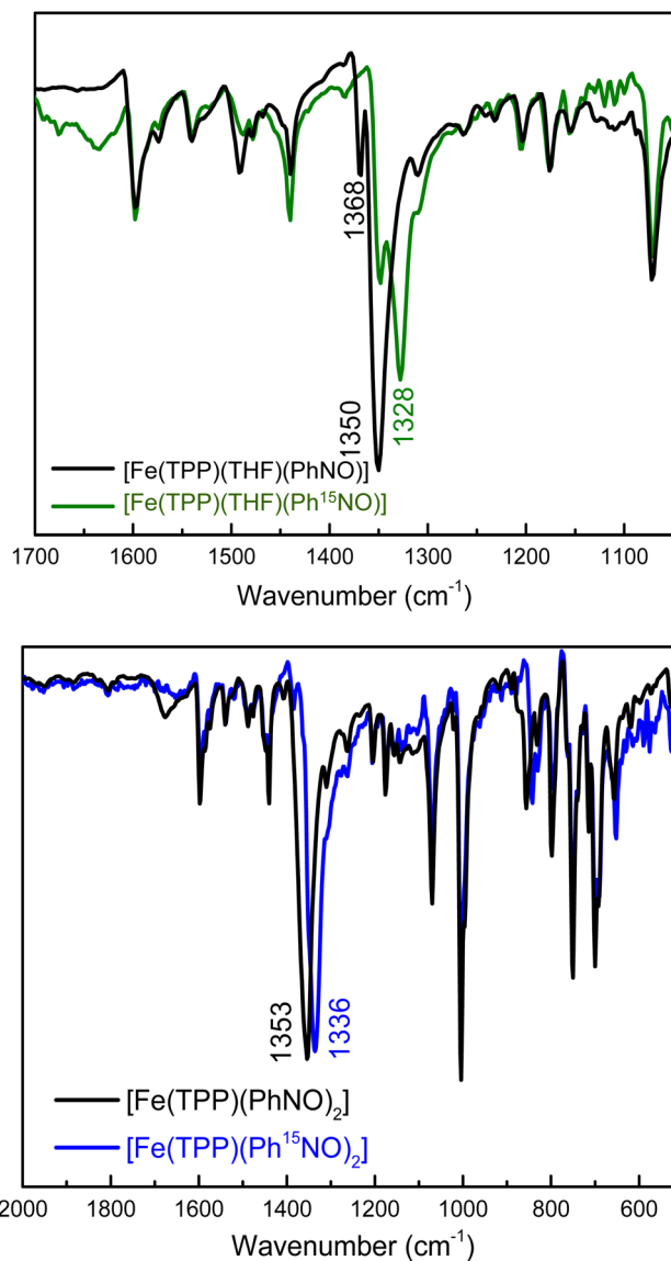
Fig. 1 Top panel: Overlay of the IR spectra of [Fe(TPP)(THF)(PhNO)] (black), and of the 15 N-labeled complex, [Fe(TPP)(THF)(Ph 15 NO)] (green), measured in KBr pellets (expanded view of the N–O stretching frequency region). Bottom panel: Overlay of the IR spectra of [Fe(TPP)(PhNO) 2 ] (black) and the 15 N-labeled complex, [Fe(TPP)(Ph 15 NO) 2 ] (blue), measured in KBr pellets. See text for further discussion.
