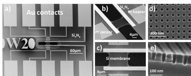
Fig. 4 (a) Seebeck coefficient measurement device illustrating the Au pads connected to the heater/sensor and the 20 μm × 20 μm Si membrane. (b) Close-up view of the suspended Si membrane and the Pt heater/sensor. (c) Top close-up view of the suspended PE Si membrane. (d) Details of the pore patterns on the Si membrane. (e) Cross-section view of the holes.
