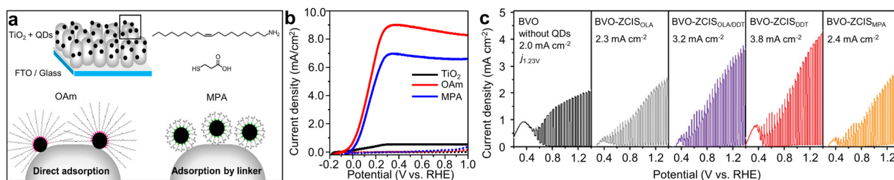
Fig. 5 Ligand modification of Cu-based I-III-VI QDs for PEC hydrogen production. (a) Schematic illustration showing the adsorption mechanisms of CISE QDs onto TiO 2 , and (b) corresponding J - V curves. Adapted with permission from ref. 56. Copyright 2022, MDPI. (c) J - V plots for photoanodes with Zn-doped CIS QDs depending on the passivation ligands. Adapted with permission from ref. 57. Copyright 2022, Wiley.
