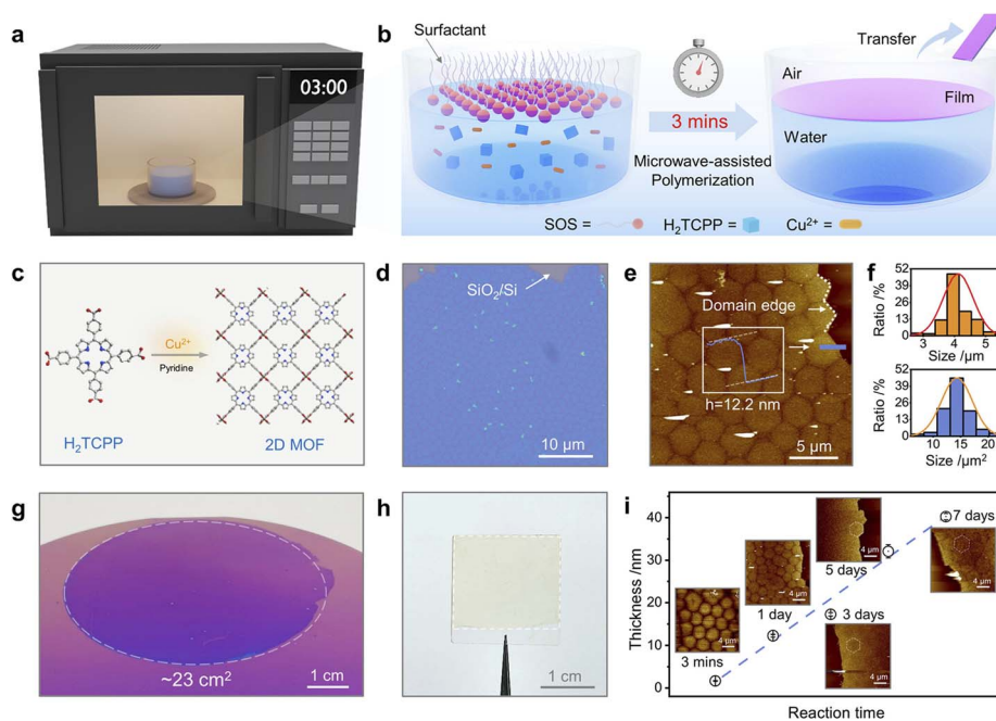
Fig. 3 Synthesis and morphology of 2D MOF thin film. (a) Illustration of the microwave oven. (b) Synthesis of a 2D MOF on the water surface. (c) Chemical structures of monomer and 2D MOF. (d) Optical microscopy image of 2D MOF after 24 h polymerisation. (e) AFM image of 2D MOF after 24 h polymerisation. (f) Statistical distribution of the domain size of the 2D MOF crystals. (g) 2D MOF film on a 300 nm SiO 2 /Si wafer (diameter Ø = 10 cm). (h) Optical microscopy image of the 2D MOF on quartz. (i) Thickness of 2D MOF vs. reaction time (inset: AFM image of the 2D MOF from 3 min to 7 days). Copyright 2023 American Chemical Society.
