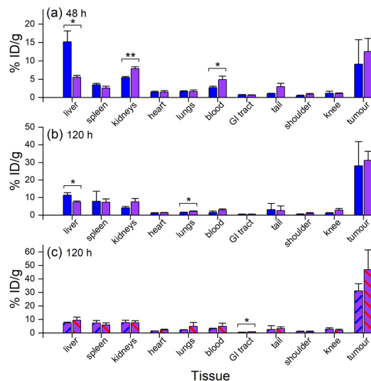
Fig. 10 Ex vivo biodistribution from gamma counting ( n = 3 ) of [ 89 Zr]Zr-1-mAb (blue) and [ 89 Zr]Zr-D2-mAb (purple) at (a) 48 h p. i. or (b) 120 h p. i., or (c) [ 89 Zr]Zr-D2-mAb (purple, blue diagonal line) and [ 177 Lu]Lu-D2-mAb (purple, red diagonal line) at 120 h p. i. * p \leq 0.05 , ** p \leq 0.01 .
