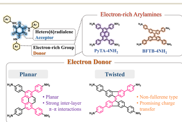
Fig. 1 Schematic representation of our principle for the design of the donor-acceptor structure with the hetero[6]radialene core as the acceptor, and planar pyrene and twisted bifuorenylidene cores as donors.
