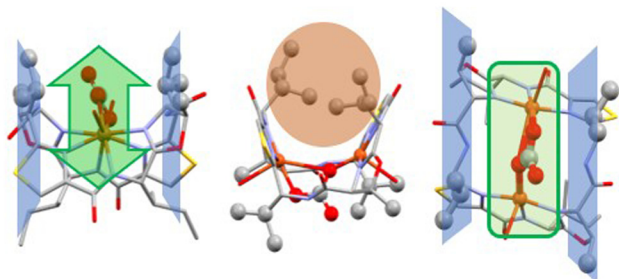
Fig. 4 Crystal structure of the dinuclear \text{Cu}^{\text{II}} complex of ascidiacyclamide, bridged by carbonate (in green). 86 The isobutyl side chains from the \text{D} -valines lie in a plane with the methyl group from the oxazolines (colored in blue), parallel to the plane containing the \text{Cu}^{\text{II}}-\text{CO}_3^{2-}-\text{Cu}^{\text{II}} site. This preorganization allows for easy access to the dinuclear copper center of small, flat or linear molecules such as carbonate/ \text{CO}_2 from one side (highlighted in green). 88
