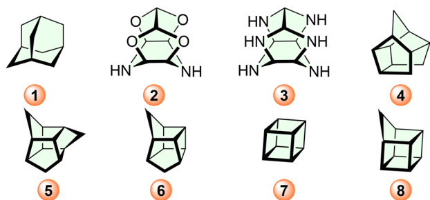
Adamantane (1). 2,6,8,12-Tetraoxa-4,10-diazatetracyclo[5.5.0.0 3,11 ].dodecane (2). 2,4,6,8,10,12-Hexaazatetracyclo[5.5.0.0 3,11 ].dodecane (3). Pentacyclo-(5.4.0.0 2,6,10,0 5,9 )-undecane (4). Pentacyclo[6.3.0.0 2,6,0 3,10,0 5,9 ]undecane (5). Pentacyclo[5.3.0.0 2,5,0 3,9,0 4,8 ]decane (6). Cubane (7). Pentacyclo[4.3.0.0 2,5,0 3,8,0 4,7 ]-nonane (8).
