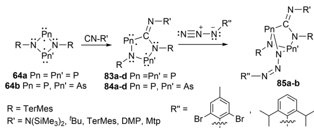
Scheme 9 Reactivity of biradicals of the type [E(\mu NTERmes)E]_2 to generate cyclopentane-1,3-diyl derivatives ( 83a-d , 84a-d ), and Staudinger-type adducts ( 85a-b ).
