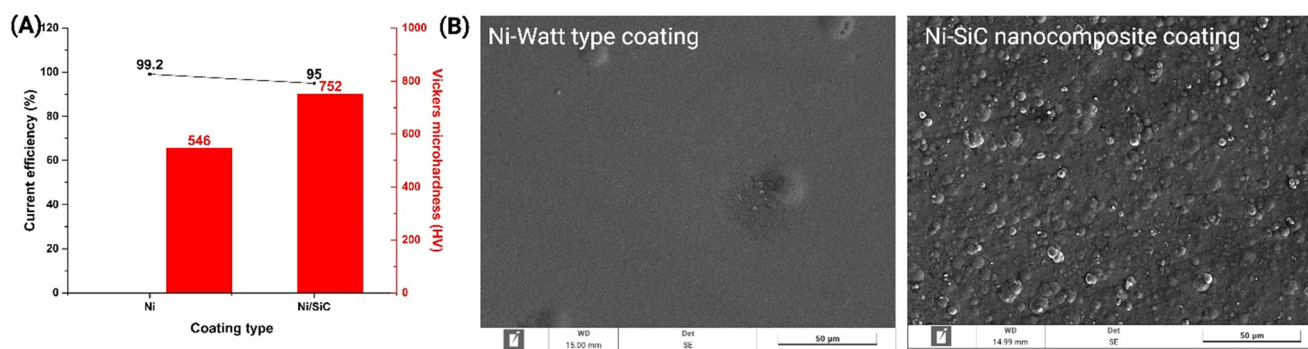
Fig. 1 Characterisation of Ni-Watts type electroplated coatings and Ni-SiC nanocomposite coatings. (A) Cathodic current efficiencies (line & symbol) and Vickers microhardness (column) of coatings deposited from the Ni-Watts type bath (Ni) and Ni-SiC bath (Ni-SiC). (B) SEM images, left: Ni-Watts type coating and right: Ni-SiC-nanocomposite coating (scale – 50\ \mu\text{m} ).
