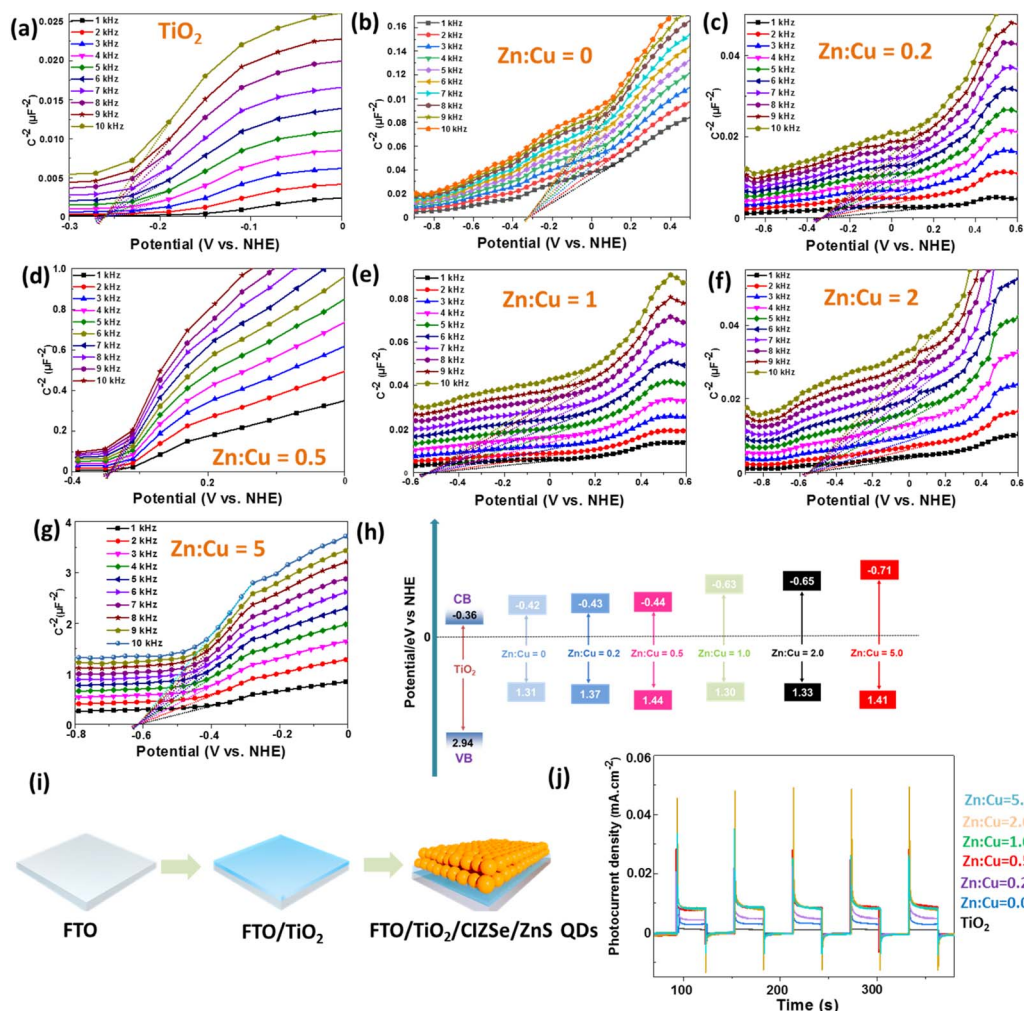
Fig. 5 (a–g) Mott–Schottky curves of \text{TiO}_2 thin film and of CIZSe/ZnS QDs (Zn : Cu = 0, 0.2, 0.5, 1, 2 and 5) deposited on FTO. (h) Electronic band structure of \text{TiO}_2 and CIZSe/ZnS QDs determined using flat band potentials and bandgap energies, (i) preparation of the FTO/ \text{TiO}_2 /CIZSe/ZnS photoelectrode, (j) transient photocurrents recorded for \text{TiO}_2 and \text{TiO}_2/\text{CIZSe/ZnS} layers on FTO (125 nm \text{TiO}_2 layer thickness, AM 1.5 G filter).
