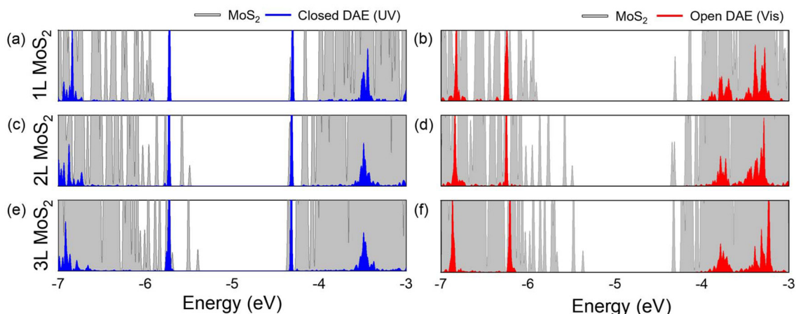
Fig. 4 DFT-calculation of density of electronic states (DOS), showing the alignment of VBM and CBM energies of 1L–3L MoS 2 with the HOMO and LUMO levels of closed- and open-form DAE under UV and visible light, respectively. The LUMO and HOMO levels of closed-form DAE are approximately -4.31 and -5.75 eV. In the open state, these values are around -3.80 and -6.32 eV, respectively. For closed-form DAE interacting with 1L MoS 2 (a), its HOMO level is higher than the MoS 2 VBM by approximately 0.16 eV. However, it is lower than the VBM levels of 2L and 3L MoS 2 by about 0.26 eV (c) and 0.36 eV (e). From (b), (d), and (f), the LUMO level is slightly higher than the CBM energies of all 1L, 2L, 3L MoS 2 by approximately 0.02 – 0.05 eV. In contrast, the HOMO level of open-form isomer is always lower than the MoS 2 VBM energies, and the LUMO is significantly higher than the CBM of 1L, 2L, and 3L MoS 2 .
