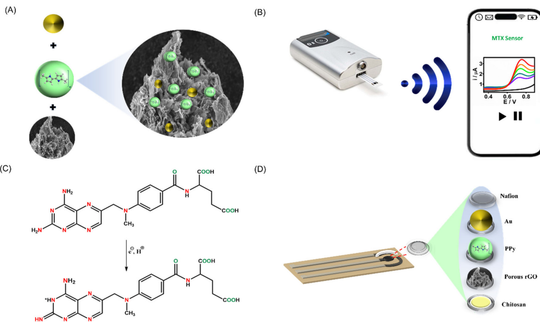
Fig. 1 Diagrams showing the synthesis and sensing process. (A) The PrGO-PPy-Au nanocomposite. (B) Recording voltammograms of methotrexate using a bluetooth-enabled handheld potentiostat and a mobile device. (C) Electrochemical oxidation behaviour of methotrexate. (D) Diagram depicting the modified SPCE sensor's layered architecture incorporating a PrGO-PPy-Au composite within a chitosan matrix and protected by a Nafion layer.
