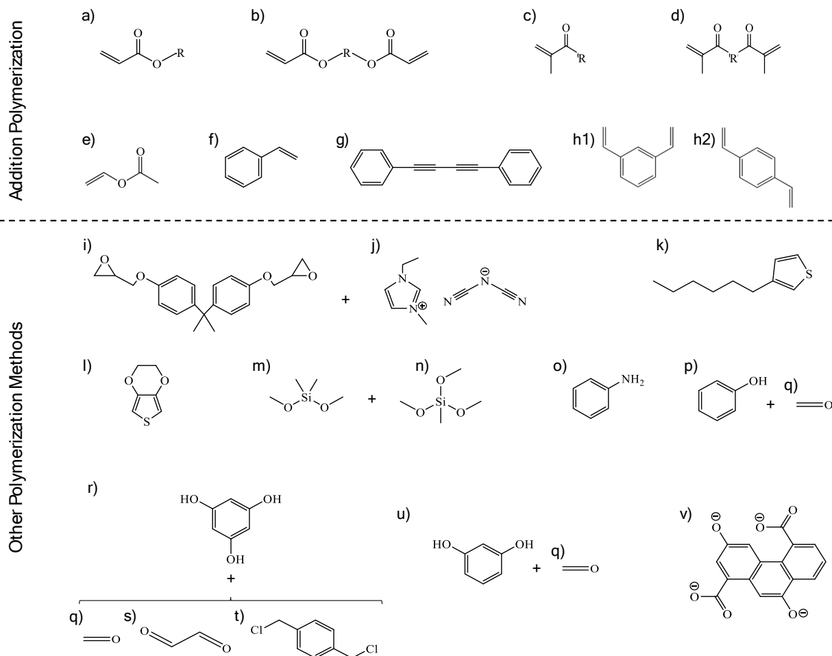
Fig. 4: Structure of the most common polymerizable groups and monomers used for polymerization in nanoconfinement: a) acrylate monomers, 26–31 b) diacrylate monomers, 28,32–36 c) methacrylate monomers, 21,24,37–39 d) dimethacrylate monomers, 40–42 e) vinyl acetate, 43 f) styrene, 44–46 g) 1,4-diphenylbutadiyne, 47 h) divinyl benzene, 48 i) bisphenol A diglycidyl ether crosslinked with j) 1-Ethyl-3-methylimidazolium dicyanamide, 49 k) 3-hexylthiophene, 50 l) 2,3-dihydrothieno[3,4-b]-1,4-dioxin, 51–53 m) dimethyldimethoxysilane crosslinked with n) methyltrimethoxysilane, 54 o) aniline, 55 p) phenol and q) formaldehyde, 56,57 r) phloroglucinol crosslinked with q) formaldehyde, 58,59 s) glyoxal, 60,61 or t) 1,4-bis(chloromethyl)benzene, 62 u) resorcinol crosslinked with q) formaldehyde, 59 and v) 3,9-dioxidophenanthrene-1,5-dicarboxylate, 63
