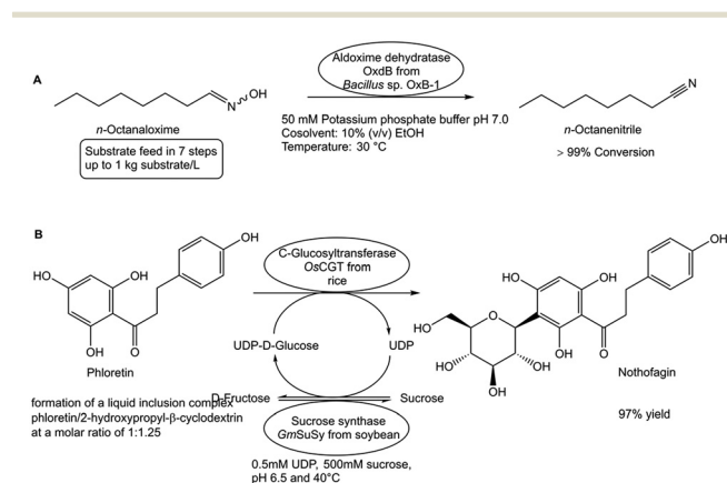
Fig. 14 Overcoming substrate solubility constraints is illustrated by two approaches. The substrate feed method has been used in the aldoxime dehydratase OxB-catalyzed dehydration of n -octanaloxime to n -octanenitrile (Fig. 14A), where the n -octanaloxime is added in seven portions to the aqueous buffer medium containing 10 % (v/v) ethanol, resulting in complete conversion of up to 1 kg L -1 substrate load. The use of suitable \beta -cyclodextrin solubilizers has been demonstrated to be superior to the cosolvent DMSO in the C-glucosyltransferase-catalyzed complete conversion of phloretin, which is \beta -D-glucosylated at its 3'-carbon; to nothofagin (Fig. 14B).
