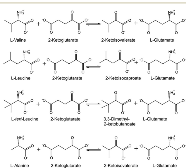
Fig. 1 Thermodynamic equilibria for transamination reactions between L -amino acid/2-ketoglutarate and the 2-ketocarboxylic acid/ L -glutamate.
