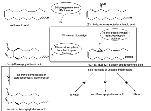
Fig. 11 Overcoming constraints of side reactions of an instable intermediate and a stereochemically labile product in the biocatalytic synthesis of cis -(+)-12-oxo-phytydienic acid. 88
