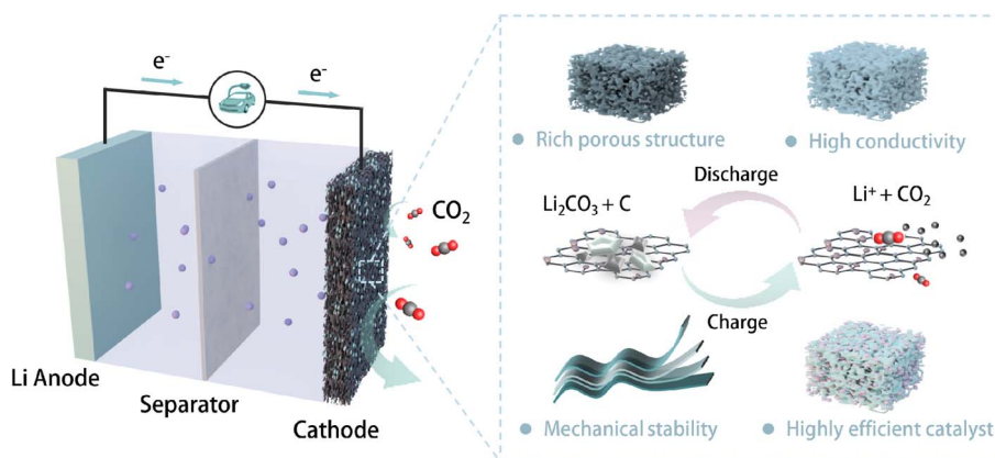
Fig. 1 Schematic illustration of a typical reversible Li– \text{CO}_2 battery structure and desirable properties for an ideal gas electrode.
