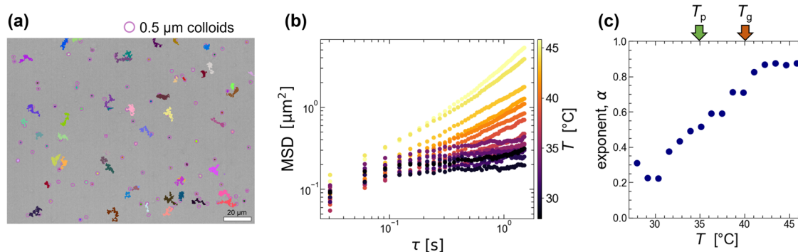
Fig. 3 (a) Microscopic image of 0.5 g/100 mL agarose with colloids after quenching at T_g = 40 ^{\circ}\text{C} . The scale bar is 20 \mu\text{m} . Pink circles with a diameter of 2.5 \mu\text{m} and the other lines indicate the positions of colloids (diameter 0.5 \mu\text{m} ) and their trajectories for 40 s, respectively. The average number density of colloids is greater than one per square of 20 \mu\text{m} sides. (b) Mean square displacement (MSD) averaged over several colloids during the slow quenching from 80 to 25 ^{\circ}\text{C} with 0.3 ^{\circ}\text{C min}^{-1} . (c) From the fitting with \text{MSD} \sim \tau^\alpha for the whole-time scale (0.03–2 s), the exponent \alpha is plotted against T . The green and red arrows show T_p = 35 ^{\circ}\text{C} and T_g = 40 ^{\circ}\text{C} , respectively.
