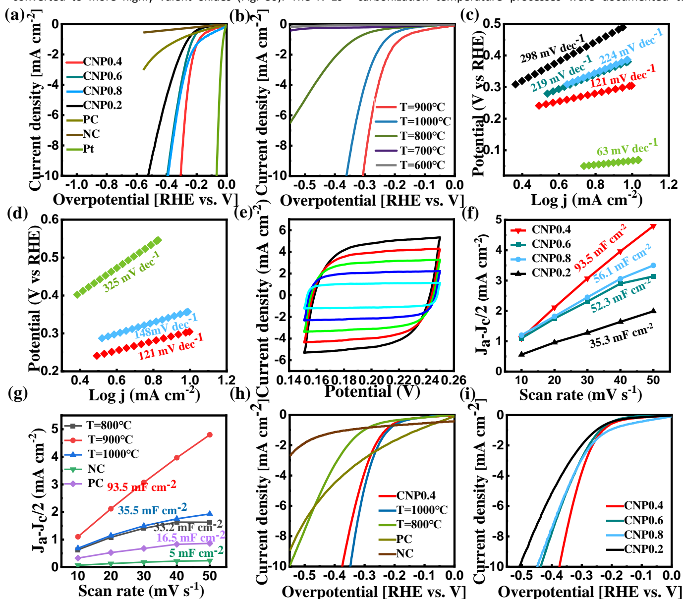
Fig 4. (a,b) The LSV curves of the various samples . (c,d) The corresponding tafel slopes. (e) The CV curves of CNP0.4 in 0.5M\ H_2SO_4 with the sweep rate changed from 10\text{ mV s}^{-1} to 50\text{ mV s}^{-1} . (f) The ESCA of sample CNP0.2, CNP0.4, CNP0.6 and CNP0.8. (g) The ESCA of sample T=800^\circ C , 900^\circ C , 1000^\circ C , PC and NC. (h) The normalized current density of sample T=800^\circ C , 900^\circ C , 1000^\circ C , PC and NC. (i) The normalized current density of CNP0.2, CNP0.4, CNP0.6 and CNP0.8.
