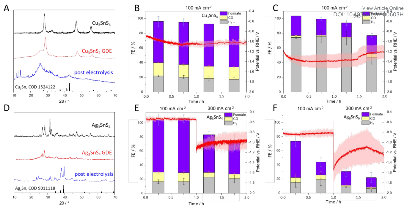
Fig. 1 Powder X-ray diffraction patterns of \text{Cu}_3\text{SnS}_4 (A) and \text{Ag}_3\text{SnS}_4 (D) as synthesized displayed in black, coated on a GDE (red) and of the GDE post-electrolysis in blue. Faradaic efficiencies obtained during \text{CO}_2\text{RR} for \text{Cu}_3\text{SnS}_4 (B) and \text{SnS} at 100 \text{ mA cm}^{-2} (C) and \text{Ag}_3\text{SnS}_4 (E) and \text{Ag}_8\text{SnS}_6 (F) at 100 \text{ mA cm}^{-2} for 1h and 300 \text{ mA cm}^{-2} for 1h. \text{CO}_2\text{RR} measurements were conducted in triplicates and standard deviations are depicted as ranges at the corresponding FE. The average of the corresponding electrode potentials in V referenced to RHE with IR correction are displayed in red, with the standard errors indicated as shaded areas.
